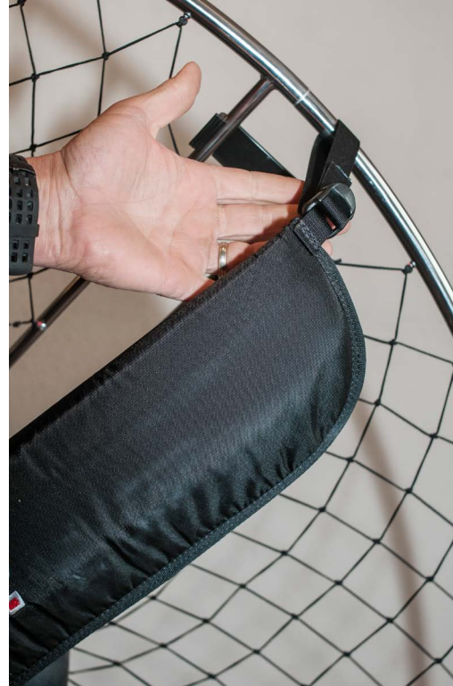
At take off, to warm the engine up, the blade can be blocked using this device. Obviously, remain on tickover so that the clutch doesn't engage, making the motor stall.
